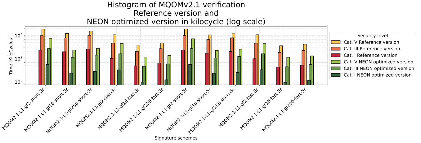
Figure 5.28: Comparison of MQOM verification algorithm, Reference and NEON versions (Table C.9)
