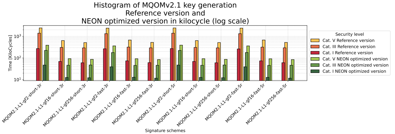
Figure 5.18: Comparison of MQOMv2.1 Key generation, Reference and NEON versions (Table C.5)
