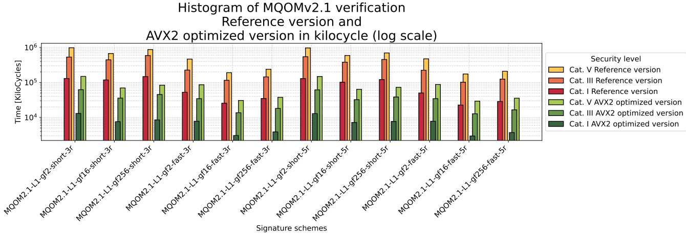
Figure 5.27: Comparison of MQOM verification algorithm, Reference and AVX2 versions (Table C.8)
