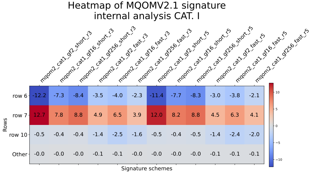
Figure 5.26: Difference in proportion (NEON - AVX2) for MQOMv2.1 signing algorithm internal analysis (Tables C.28, C.29)
