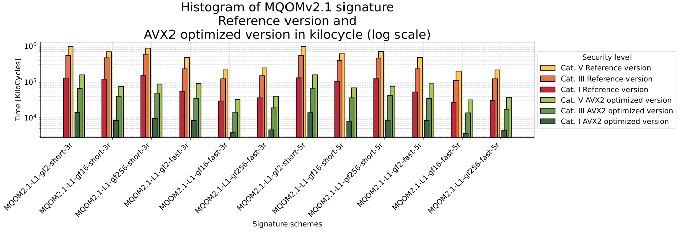
Figure 5.22: Comparison of MQOMv2.1 signing algorithm, Reference and AVX2 versions (Table C.6)
