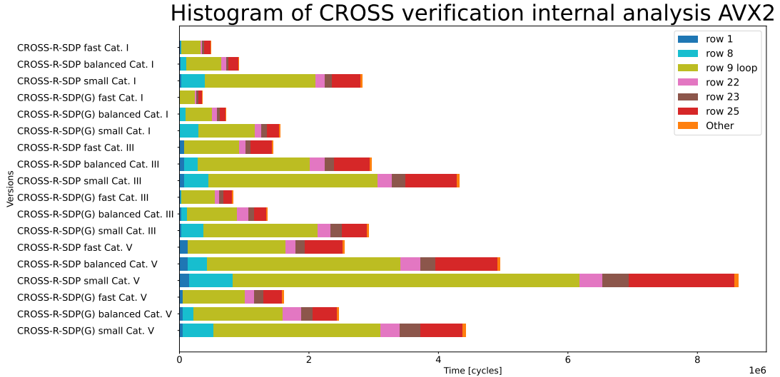
Figure 3.14: CROSS internal analysis of verification algorithm for AVX2 implementation (Tables C.16, C.17)
