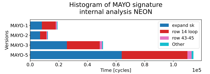
Figure 4.9: MAYO internal analysis of signing algorithm for NEON implementation (Table C.23)
