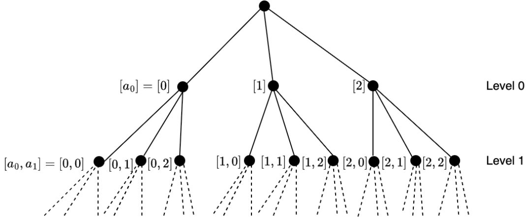
Figure 1: Tree \mathbb{T}_p corresponding to \mathbb{Z}_p ( p = 3 ), has infinite number of levels k \in \{0, 1, \dots\} . The dashed lines connect to the next level (not shown). Leaves correspond to the p -adic integers and are not shown since their level k = \infty .
