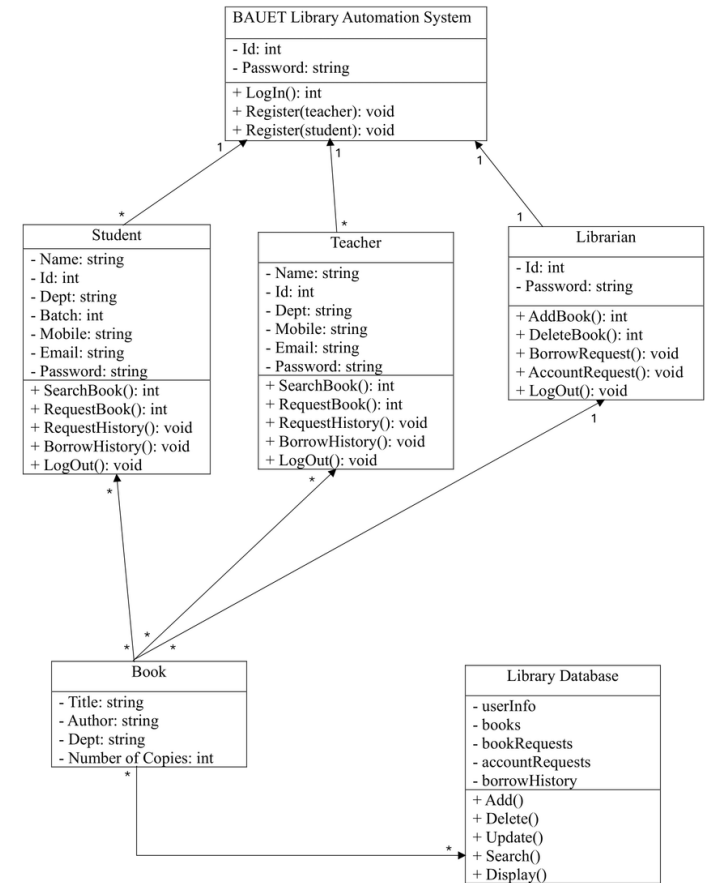
Fig: UML Diagram of BAUET Library Automation System
