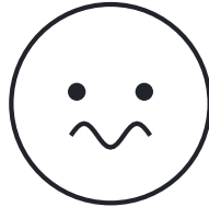
Upset
