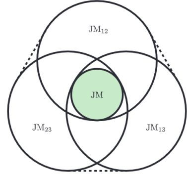
Figure 2: Convex-combination view of joint measurability for three noisy measurements, reproduced from Quintino et al. [5]: the family is jointly measurable iff it lies in the convex hull (shaded) of single-branch sub-families. JM illustrates the set of fully jointly measurable families of MUBs, while JM_{12}, JM_{13}, JM_{23} represent the sets of fully jointly measurable families for the respective pairs of measurements.
