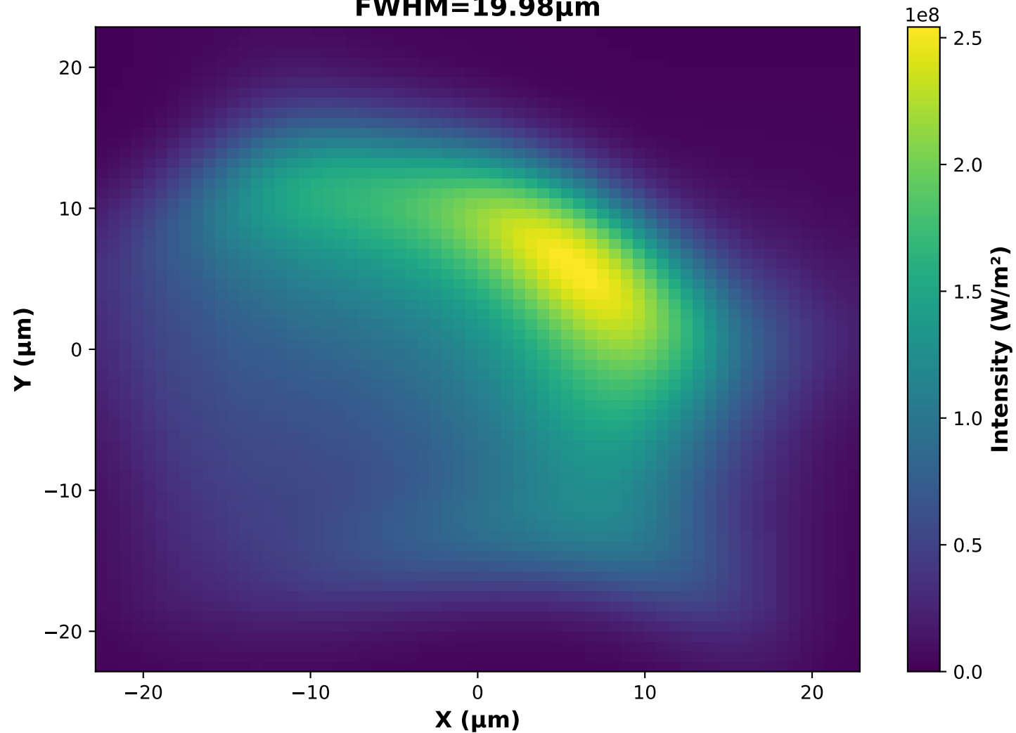
Final Profile - Simulation 1 (Seed: 1000) FWHM=19.98 \mu\text{m}
