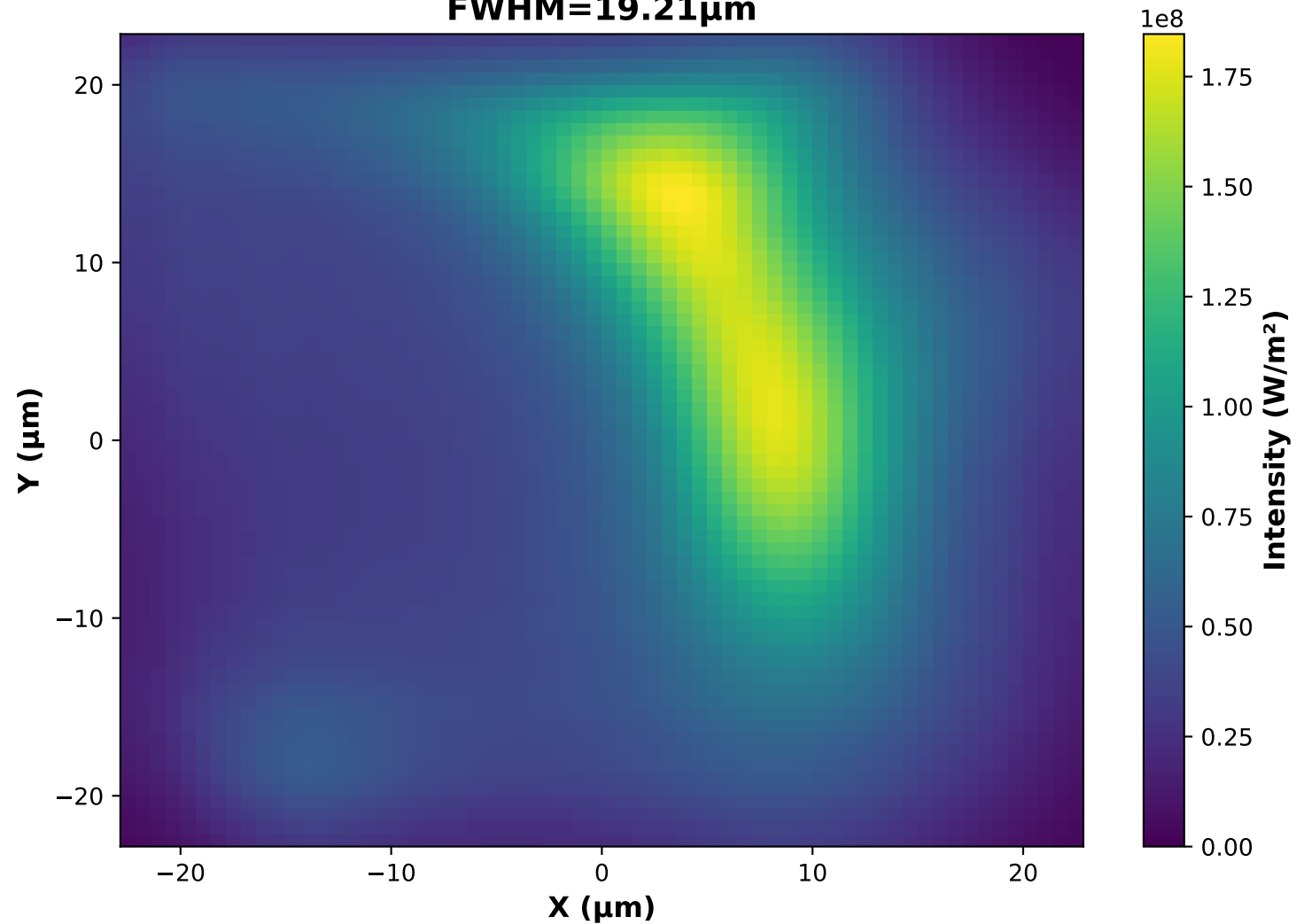
Final Profile - Simulation 2 (Seed: 2000) FWHM=19.21 \mu\text{m}
