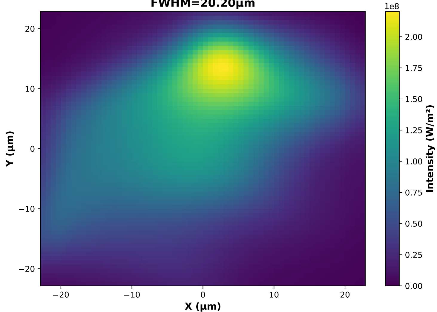
Final Profile - Simulation 3 (Seed: 3000) FWHM=20.20 \mu\text{m}
