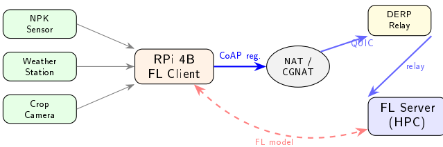
Figure 3: FL-Iroh deployment in agricultural IoT. Field sensors feed the FL client (Raspberry Pi), which registers via CoAP and exchanges model parameters over Iroh/QUIC with automatic fallback to DERP relay under NAT/CGNAT.
