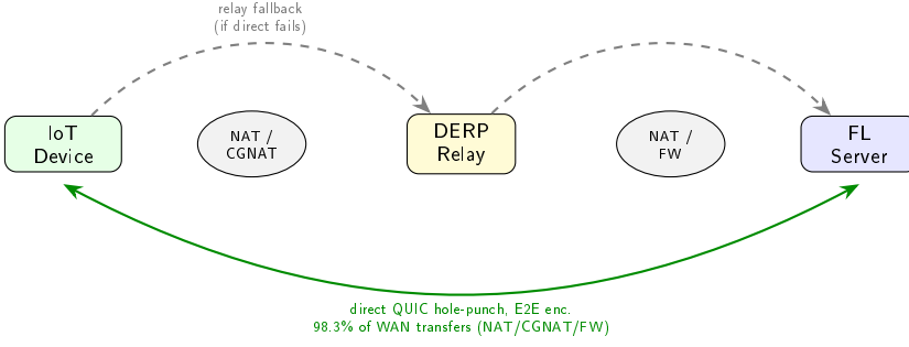
Figure 1: NAT traversal in FL-Iroh. Direct QUIC hole-punching is attempted first and, in our WAN tests, succeeds even under CGNAT and port-443 firewalls (green, end-to-end encrypted). The DERP relay remains a guaranteed fallback (grey dashed), used only if a direct path cannot be formed; the application is unaware of which path is active.
