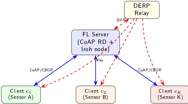
Figure 2: FL-Iroh architecture. CoAP handles service discovery and round control (blue). Iroh/QUIC carries tensor data with transparent relay fallback (red dashed) when direct hole-punch fails.
