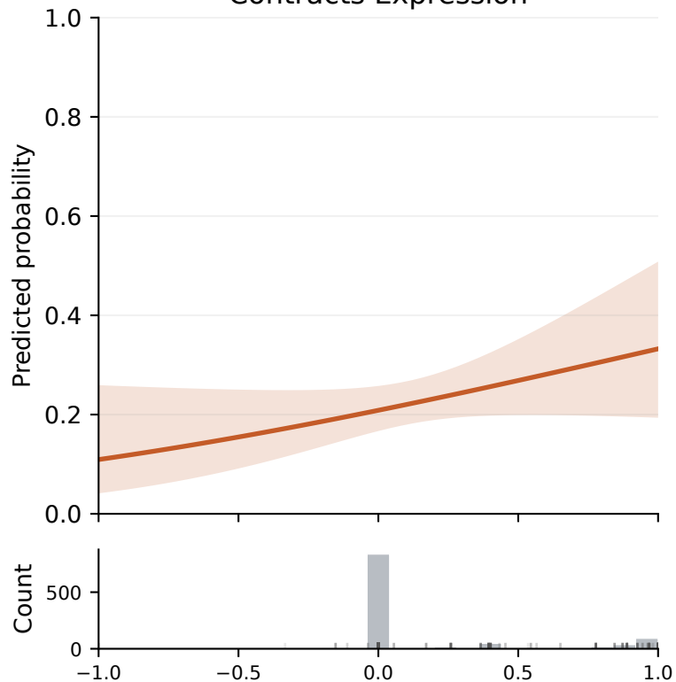
Contracts Expression
