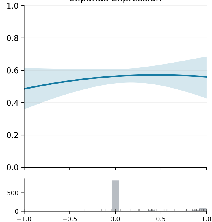
Expands Expression
