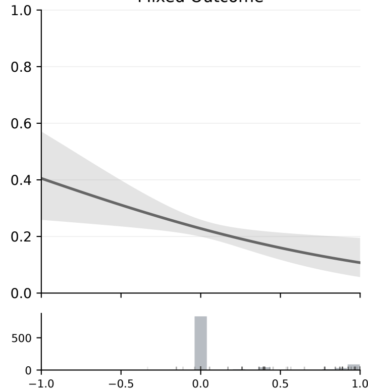
Mixed Outcome
