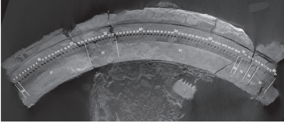
Figure 1: X-ray image of the surviving fragments of the Antikythera Mechanism.
