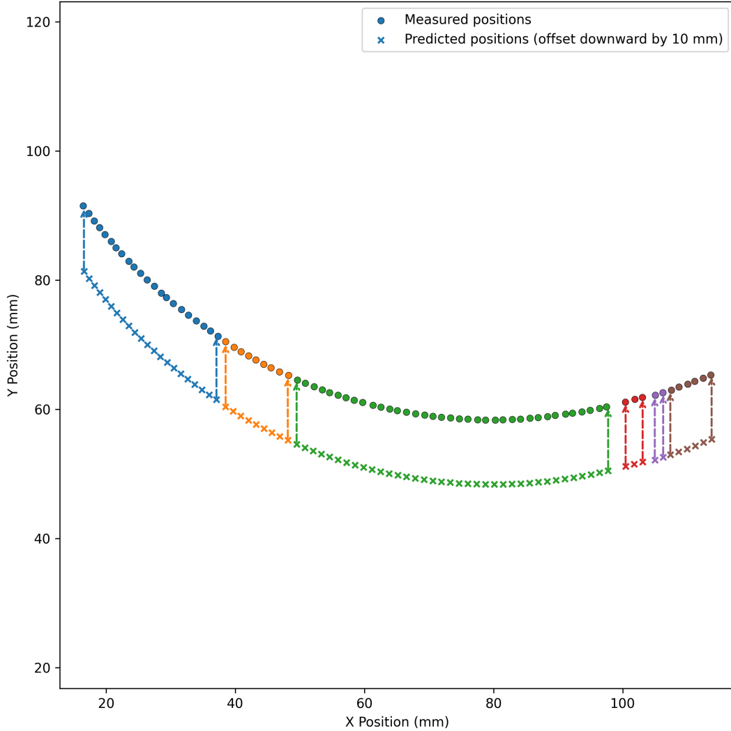
Figure 4: Measured hole positions overlaid with predicted positions from the anisotropic model, vertically shifted by 10 mm for clarity. Arrows connect the first and last predicted points in each section to their true model locations. MLE estimation: N = 355.138 , R = 77.320 .
