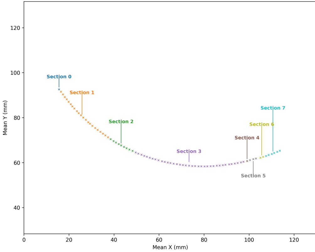
Figure 2: Measured hole locations d_i \in \mathbb{R}^2 in the x - y plane, colour-coded by fractured ring segment. Section labels are placed to minimise overlap and connected to the median point of each segment.
