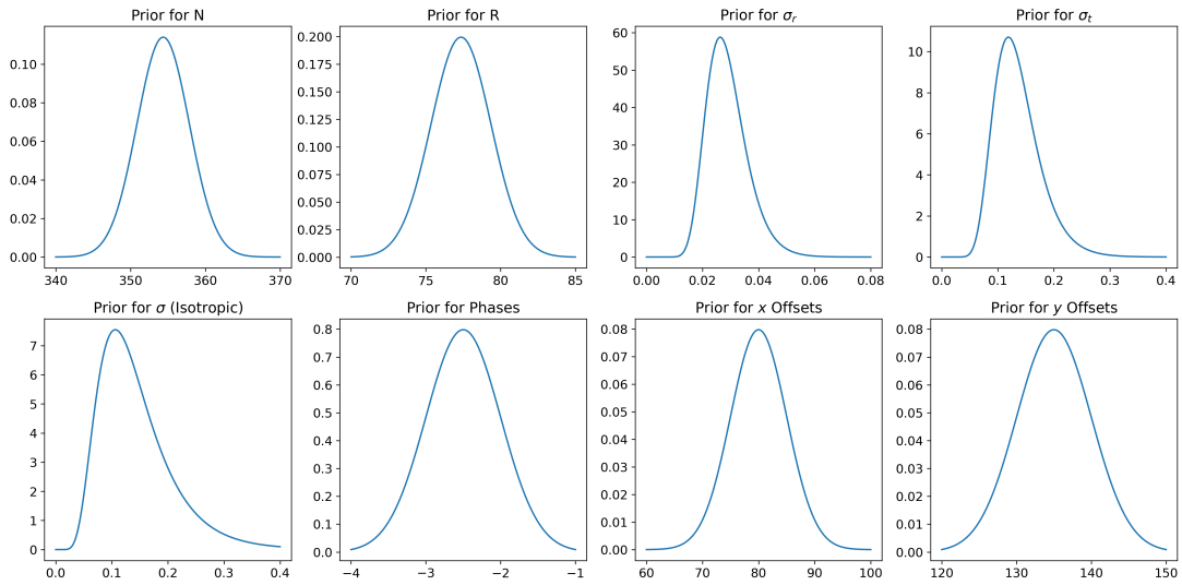
Figure 6: Prior distributions for model parameters.
