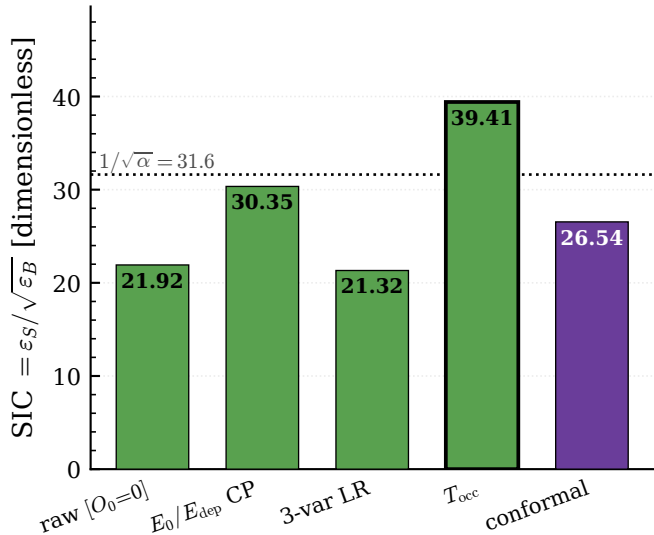
(b) Occupancy ladder ( z = 1.24 m, 5 GeV)
