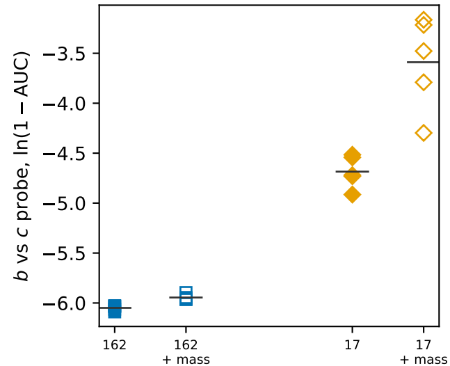
classification (frozen linear probe)
