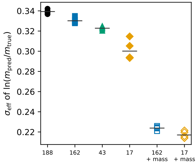
jet-mass regression (frozen ridge probe)
