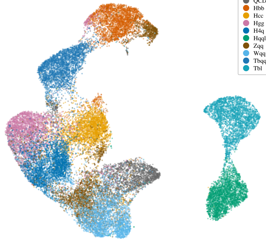
ParT-full
