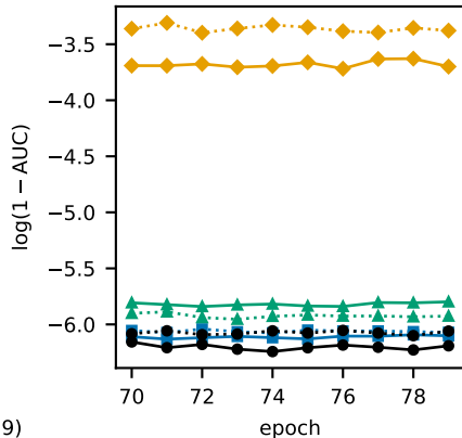
(b) linear probe, X \rightarrow b\bar{b} vs X \rightarrow c\bar{c}
