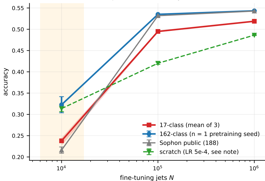
in-domain JetClass-II, 162-way
