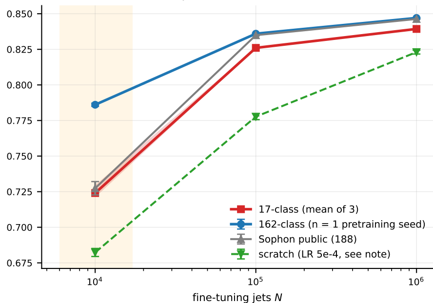
domain shift JetClass-I, 10-class
