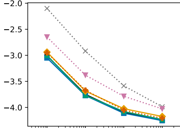
JetClass, 10 classes
