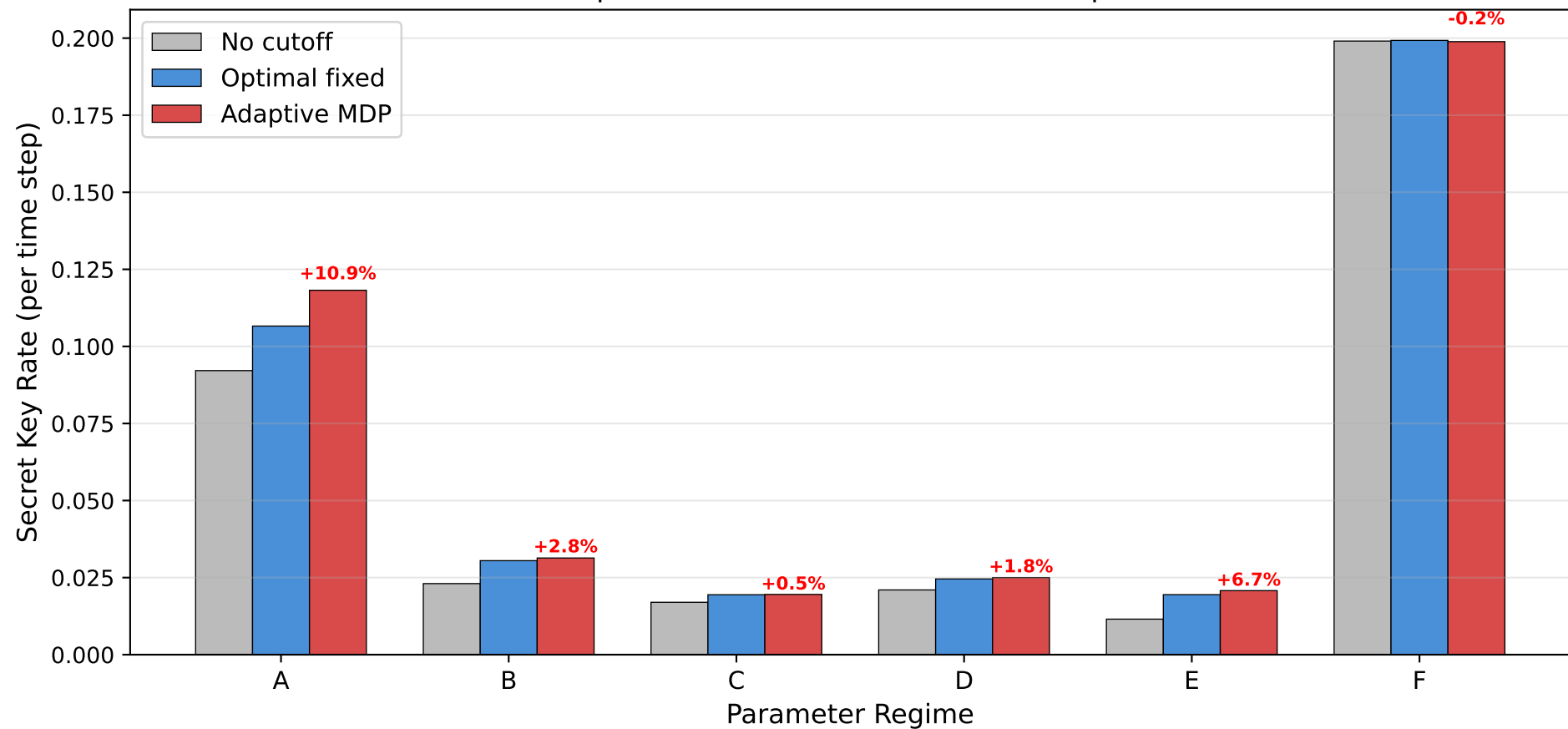
SKR Comparison: No Cutoff vs Fixed vs Adaptive MDP
