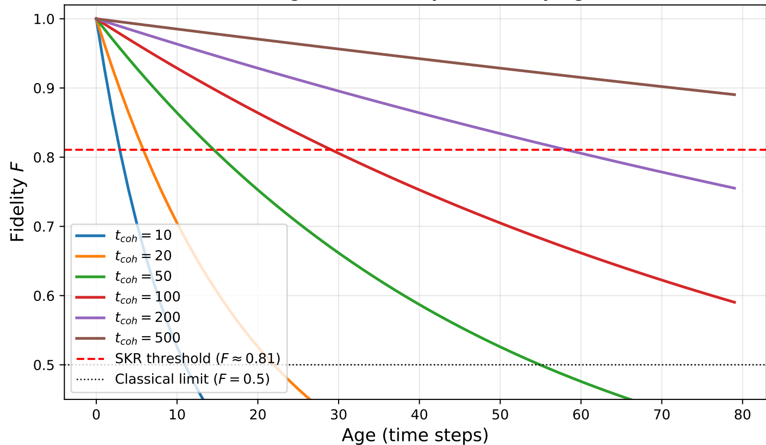
Entanglement Fidelity vs Memory Age
