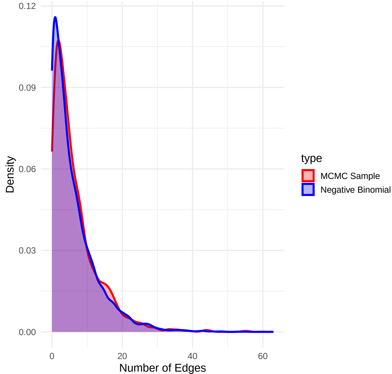
MCMC Sample vs. Negative Binomial
