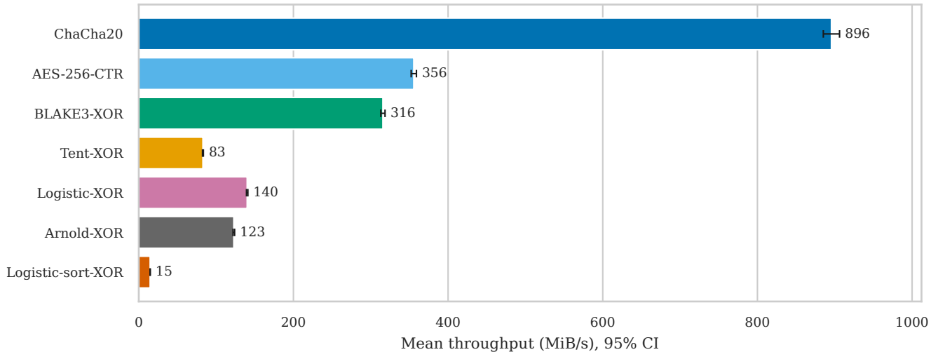
Full-scheme throughput on the 24-image Kodak dataset (768x512)
