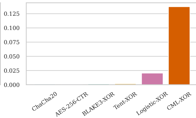
Reused-keystream KPA recovery score
