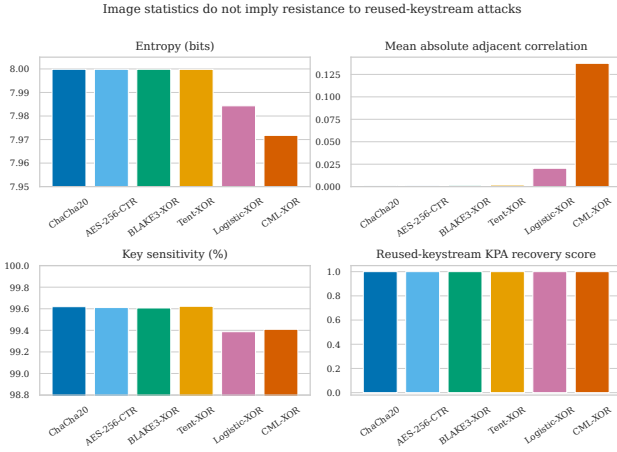
Fig. 6 Selected security diagnostics averaged over the full-scheme experiments. Near-ideal entropy, correlation, and key sensitivity coexist with complete recovery in the deliberately reused-keystream known-plaintext probe.
