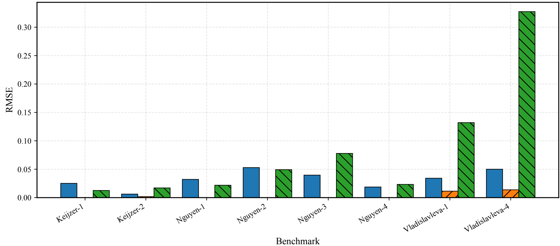
RMSE Comparison Across Benchmarks
