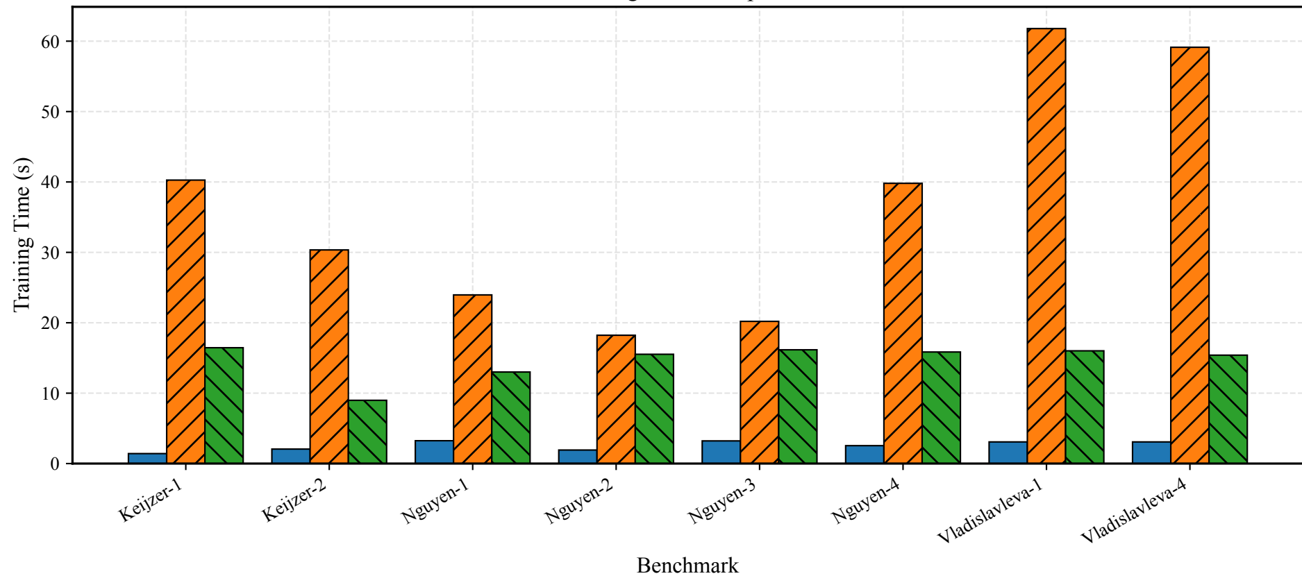
Training Time Comparison
