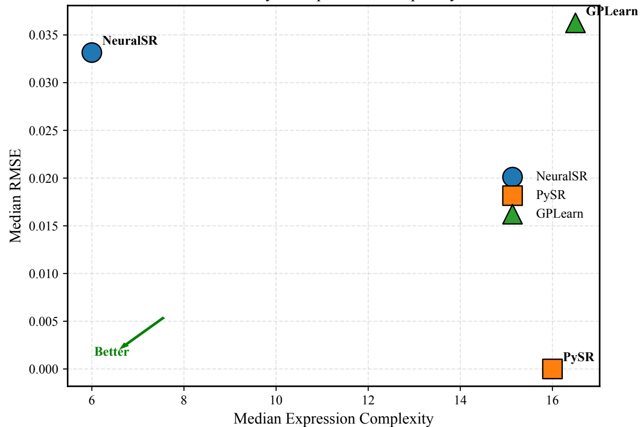
Accuracy vs Expression Complexity
