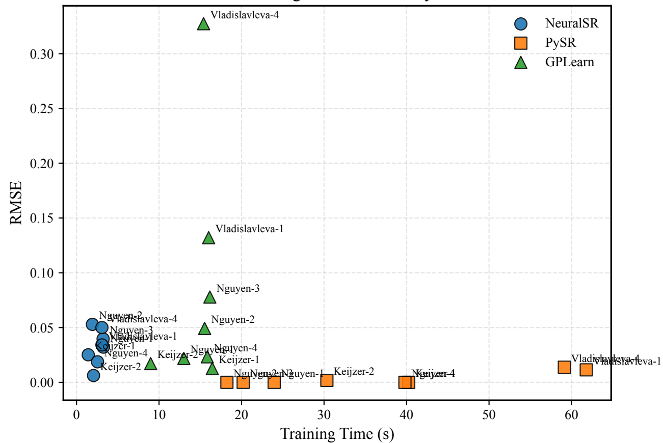
Training Time vs Accuracy
