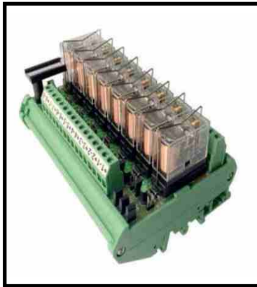
Relay Card
