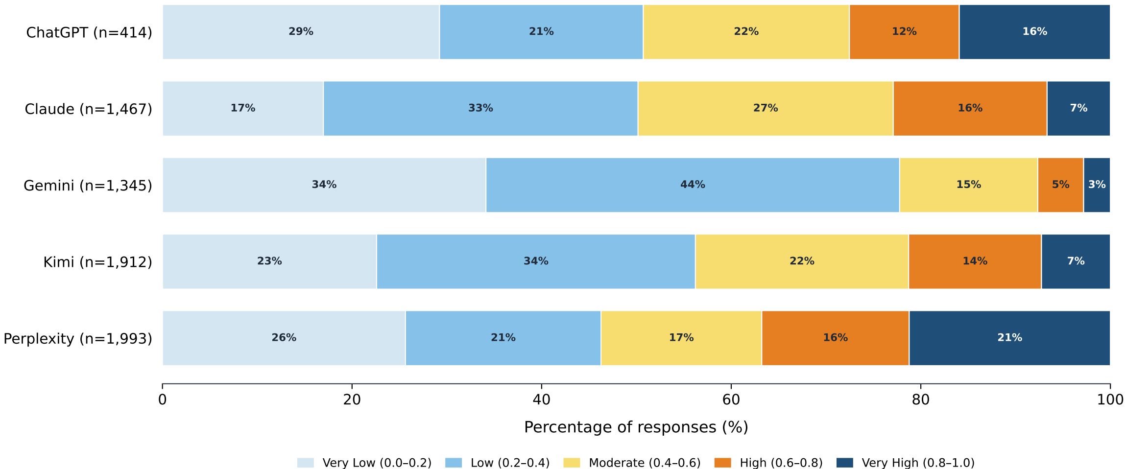
Distribution of Normalised Source Prominence (PAWC_norm) by Engine
