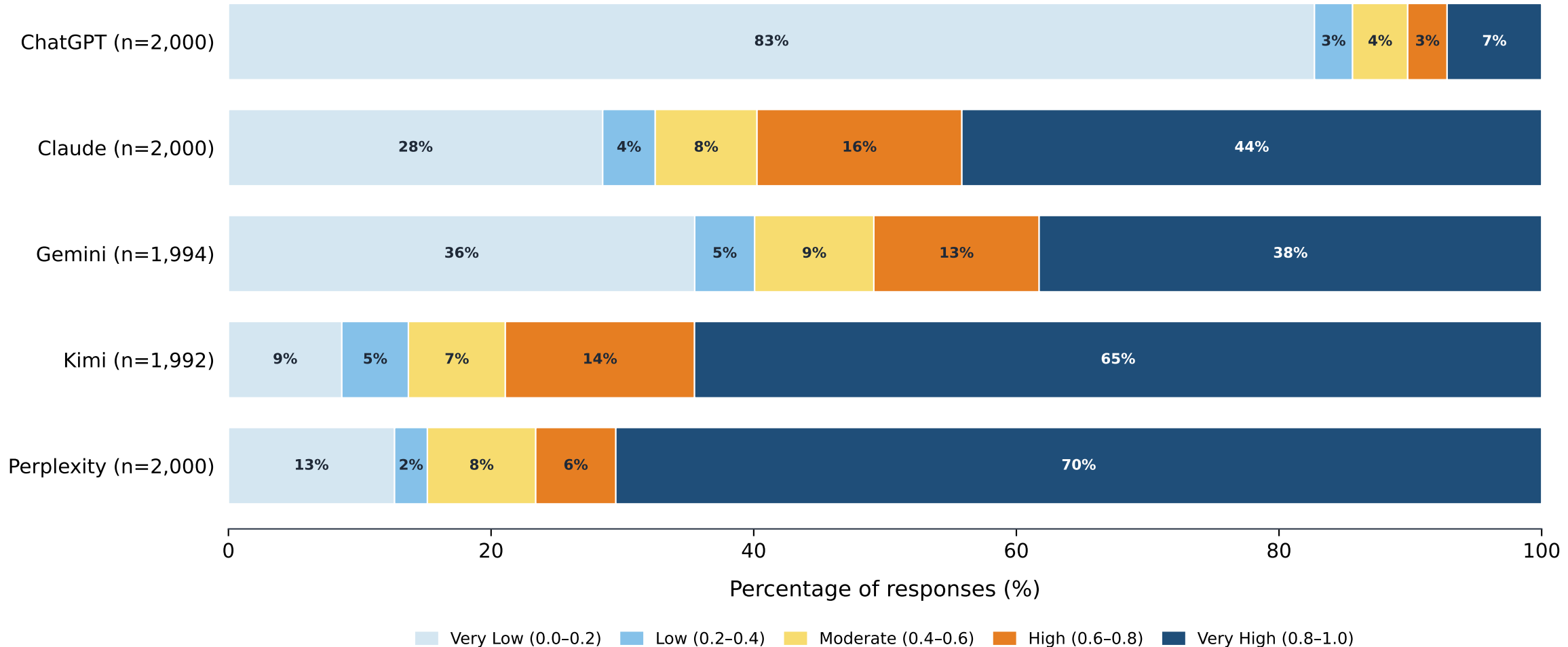
Distribution of Attributable-to-Identified-Sources rate (AIS) by Engine
