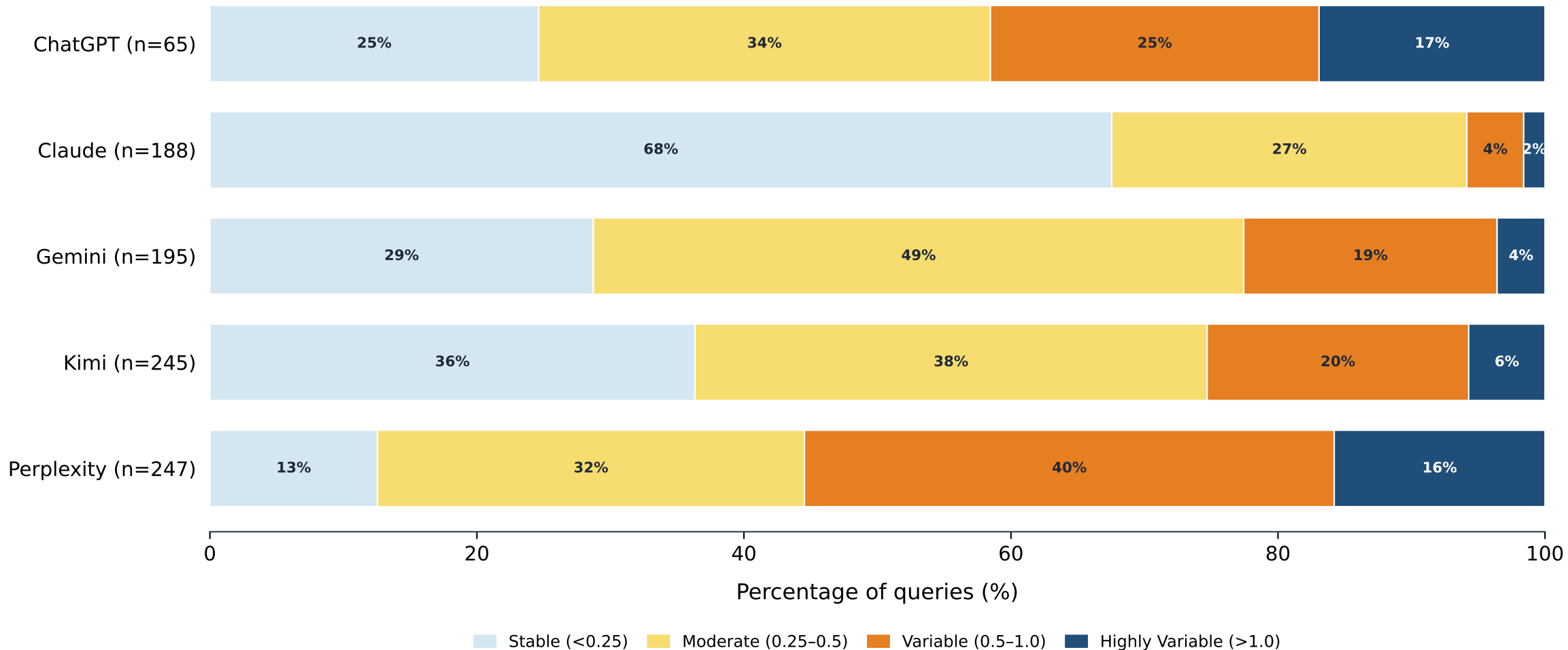
Distribution of PAWC_norm CV by Engine (k=8 runs)
