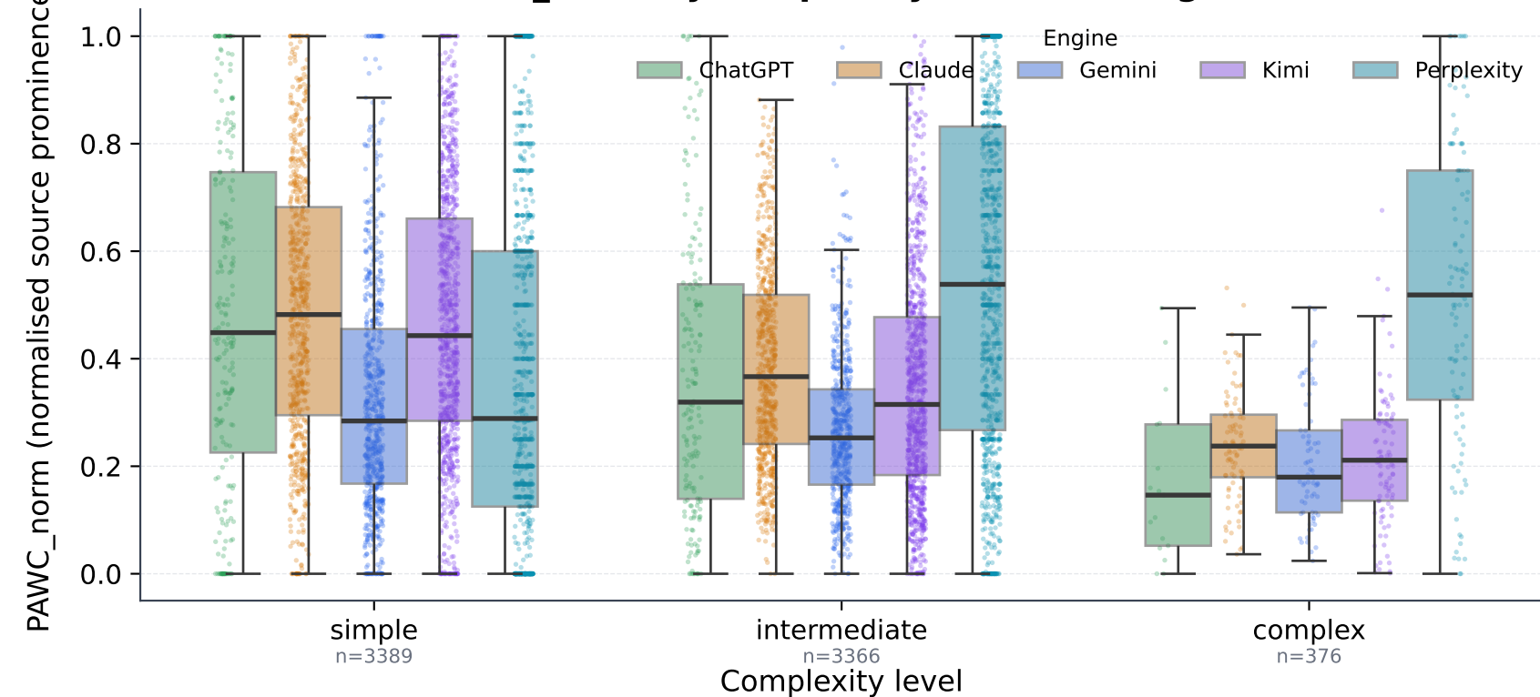
PAWC_norm by complexity level and engine
