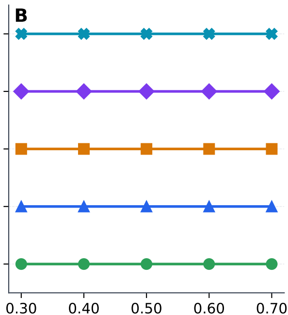
AIS rank
