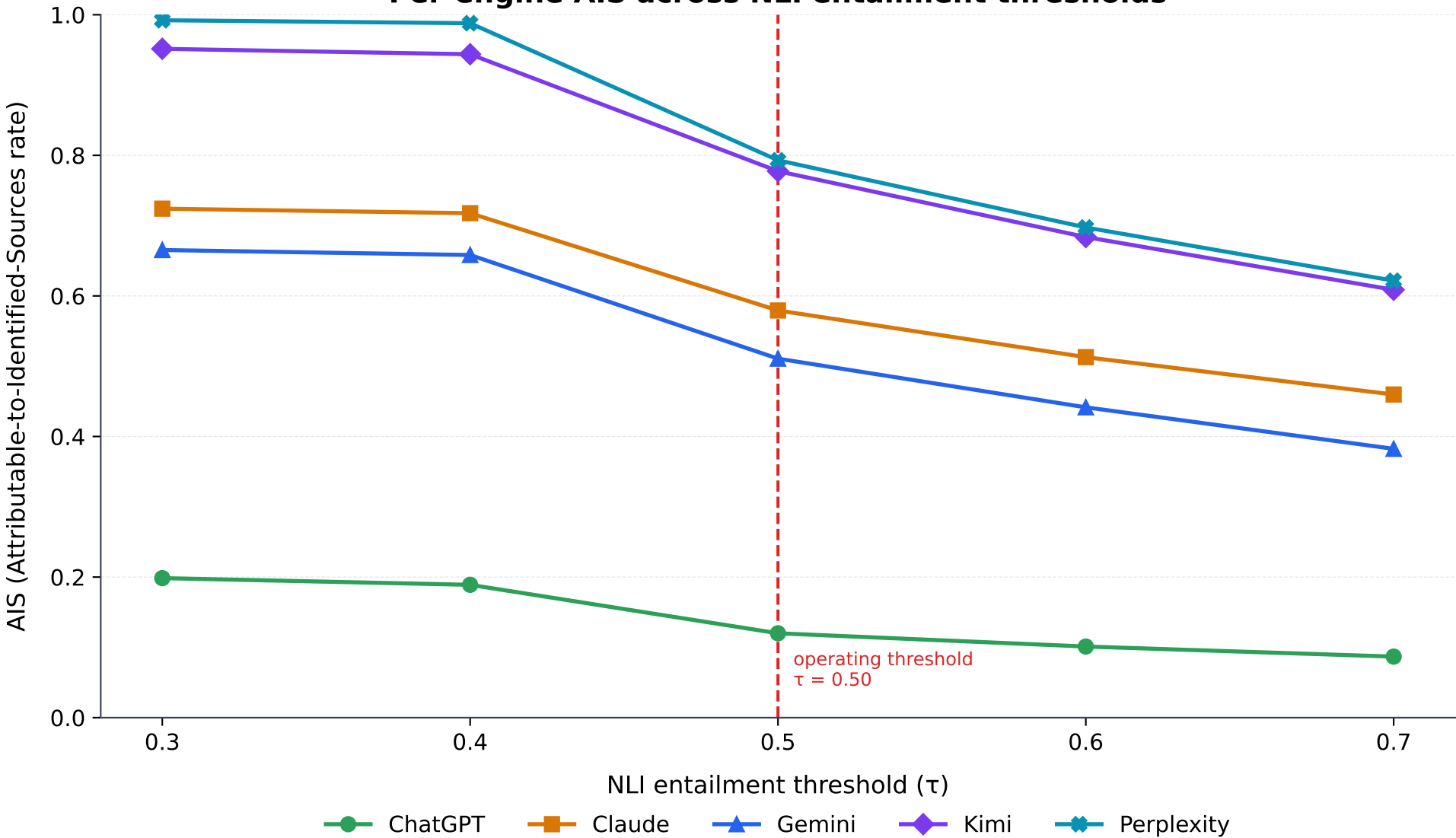
Per-engine AIS across NLI entailment thresholds
