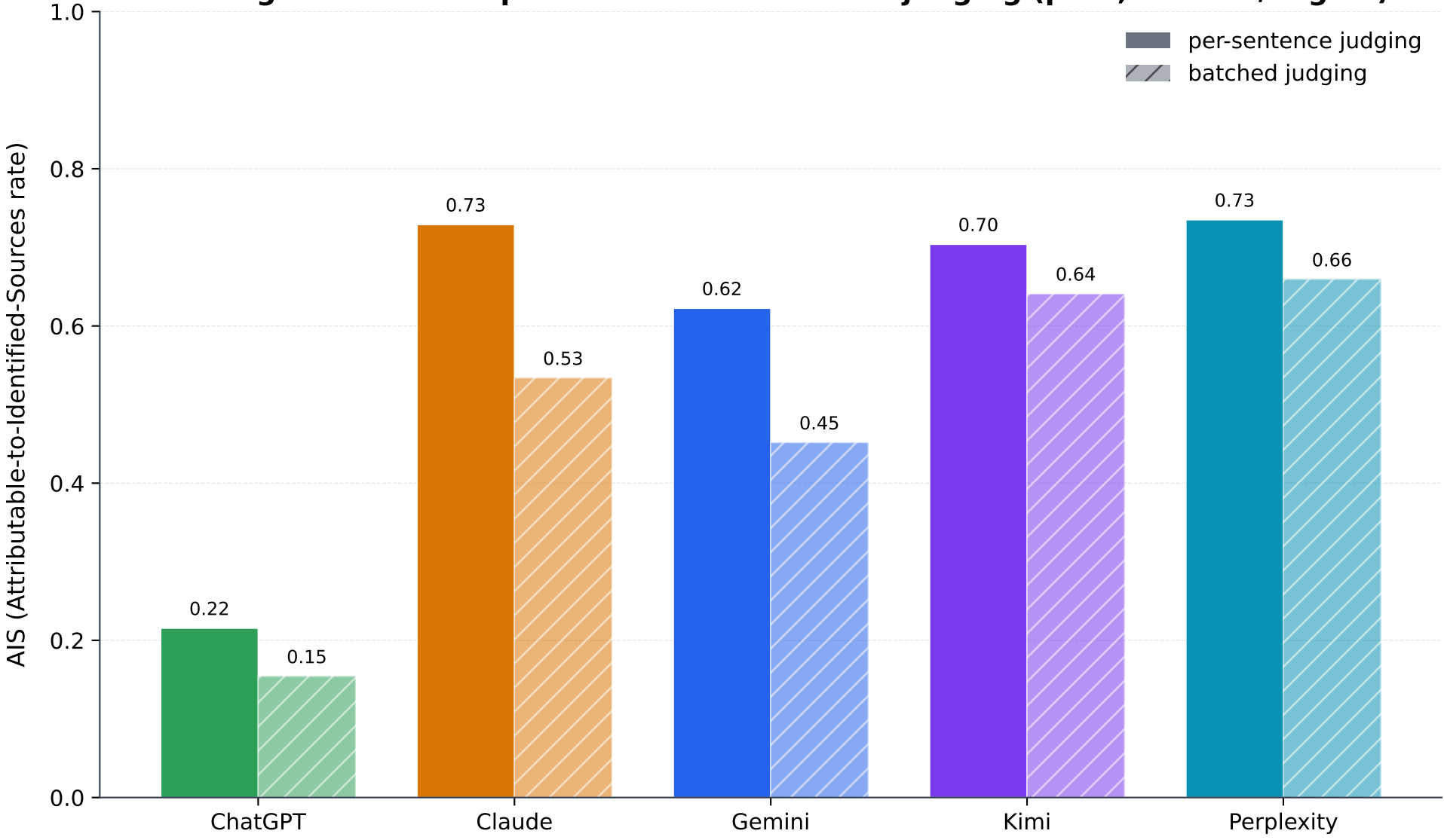
Per-engine AIS under per-sentence vs batched judging (pilot, 10 cells/engine)
