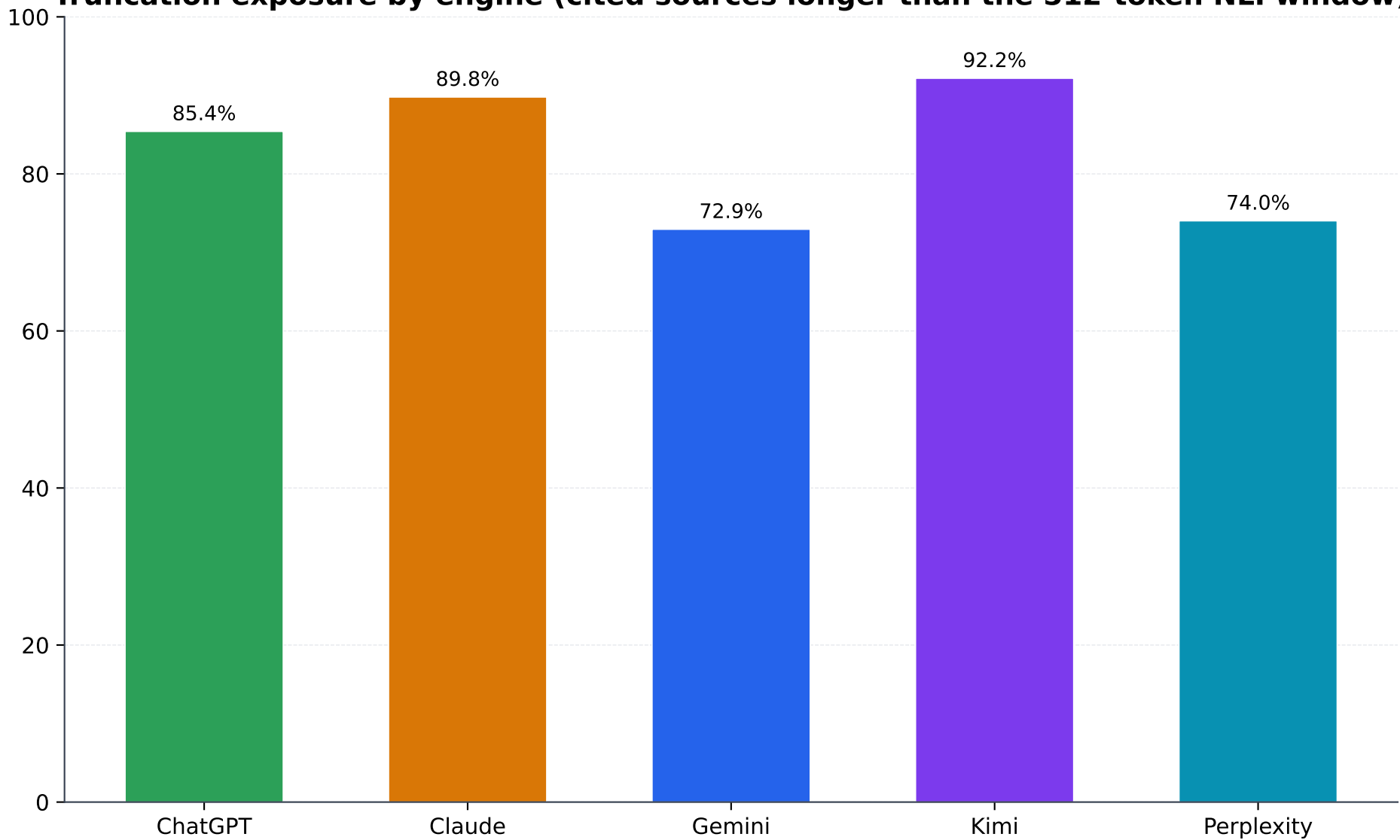
Truncation exposure by engine (cited sources longer than the 512-token NLI window)
