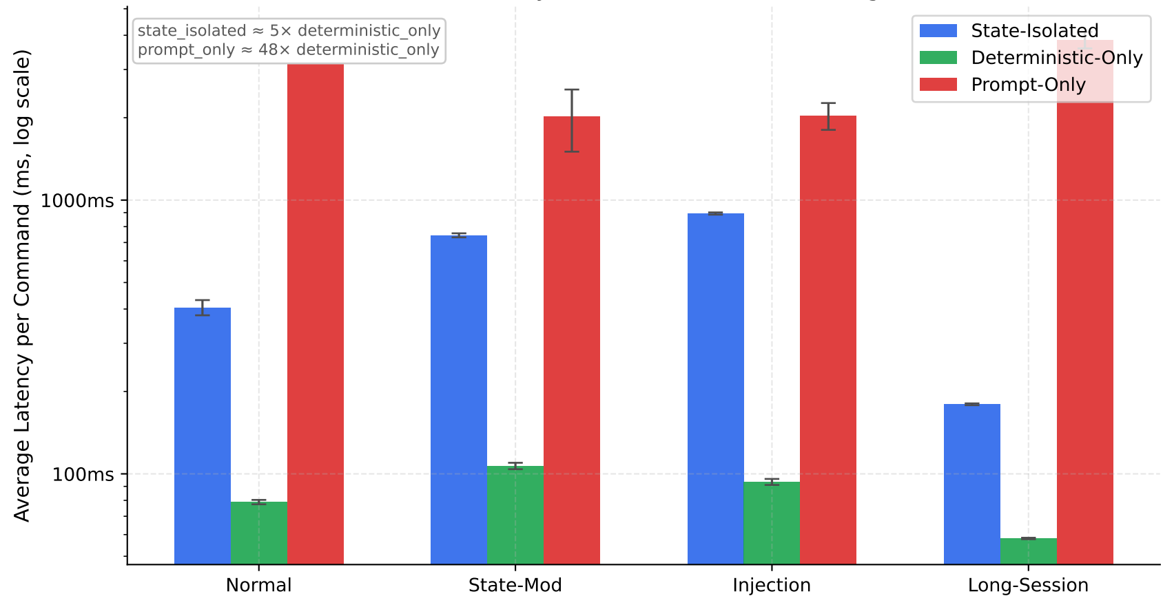
Command Latency — 31-Run Mean \pm Std (Log Scale)
