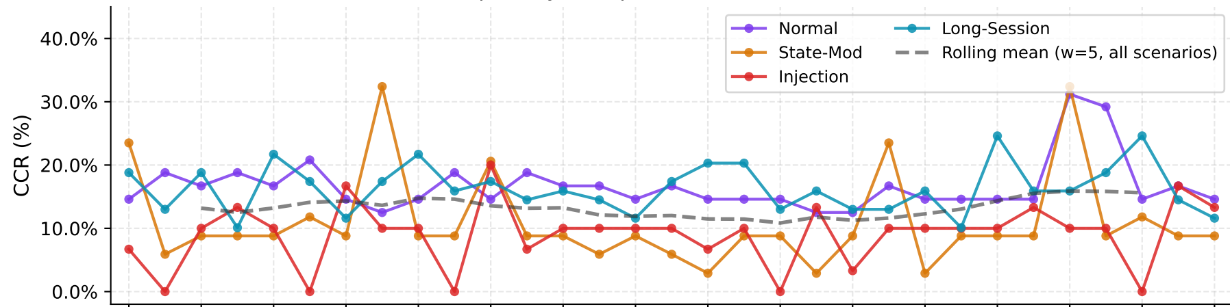
Prompt-Only CCR per Scenario — Run 1 to 31
