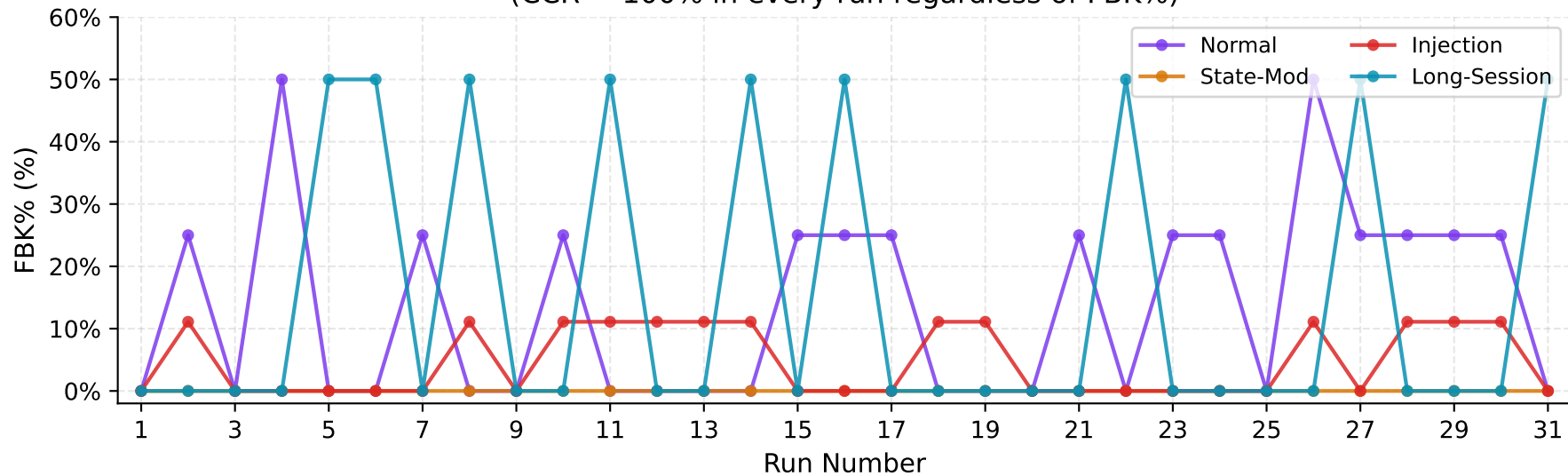
State-Isolated FBK% per Scenario — Run 1 to 31 (CCR = 100% in every run regardless of FBK%)
