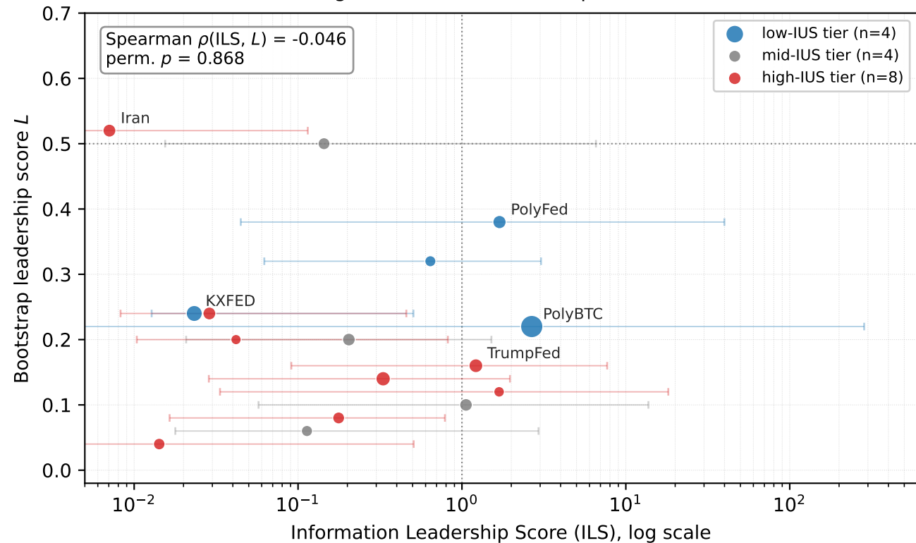
Pre-registered 16-market IUS panel: ILS vs L
