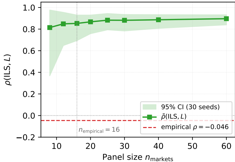
(b) Panel-size sweep, \beta = 0.30
