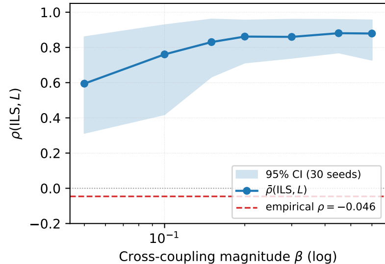
(a) Effect-size sweep, n_{\text{markets}} = 16
