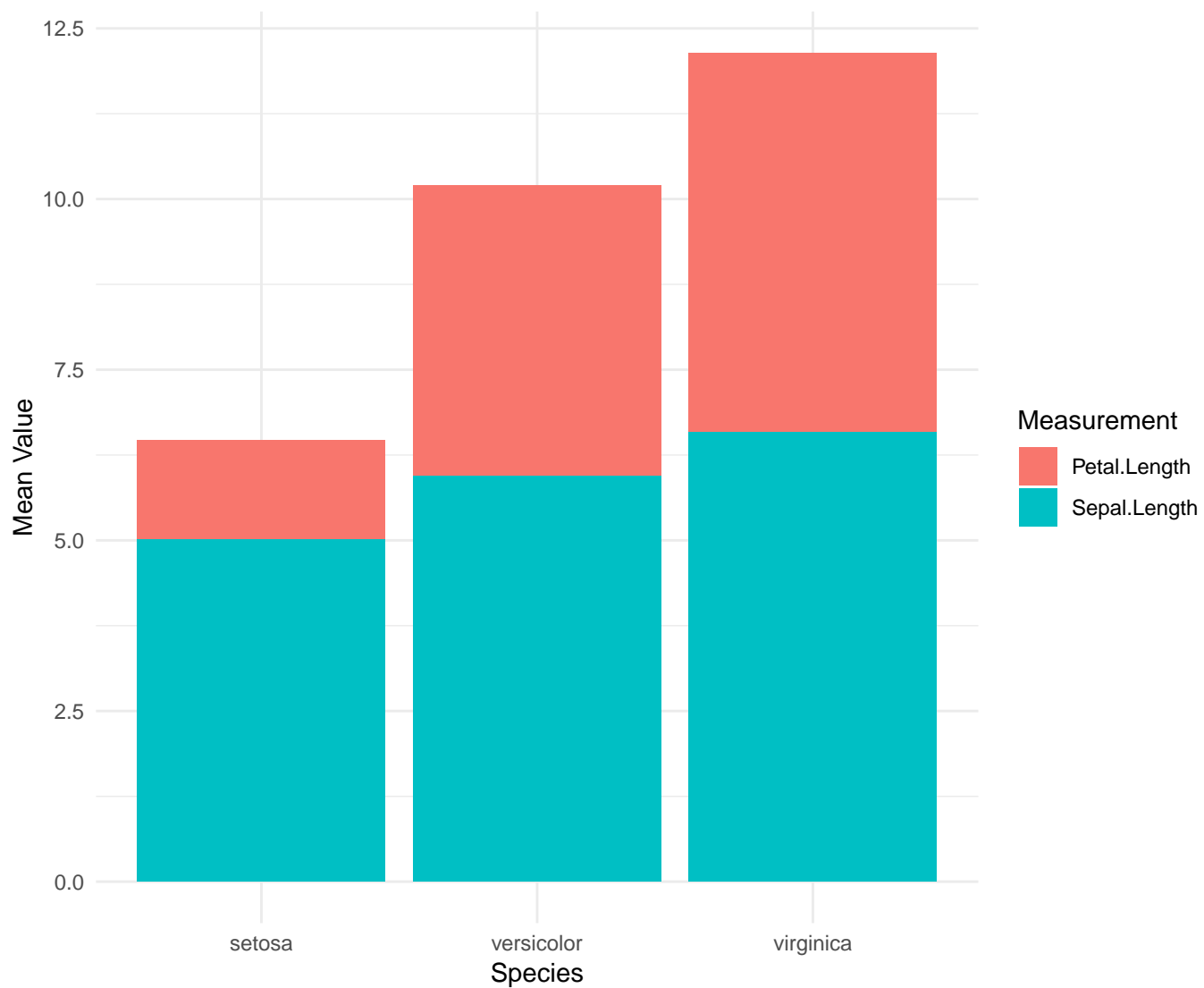
Stacked Bar Chart of Mean Measurements (Iris)
