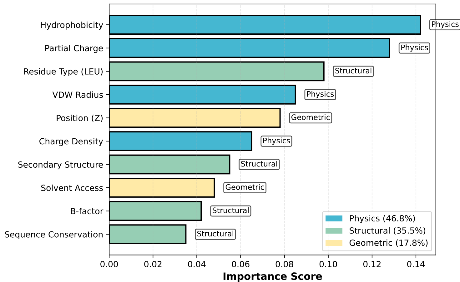
Top Feature Importance
