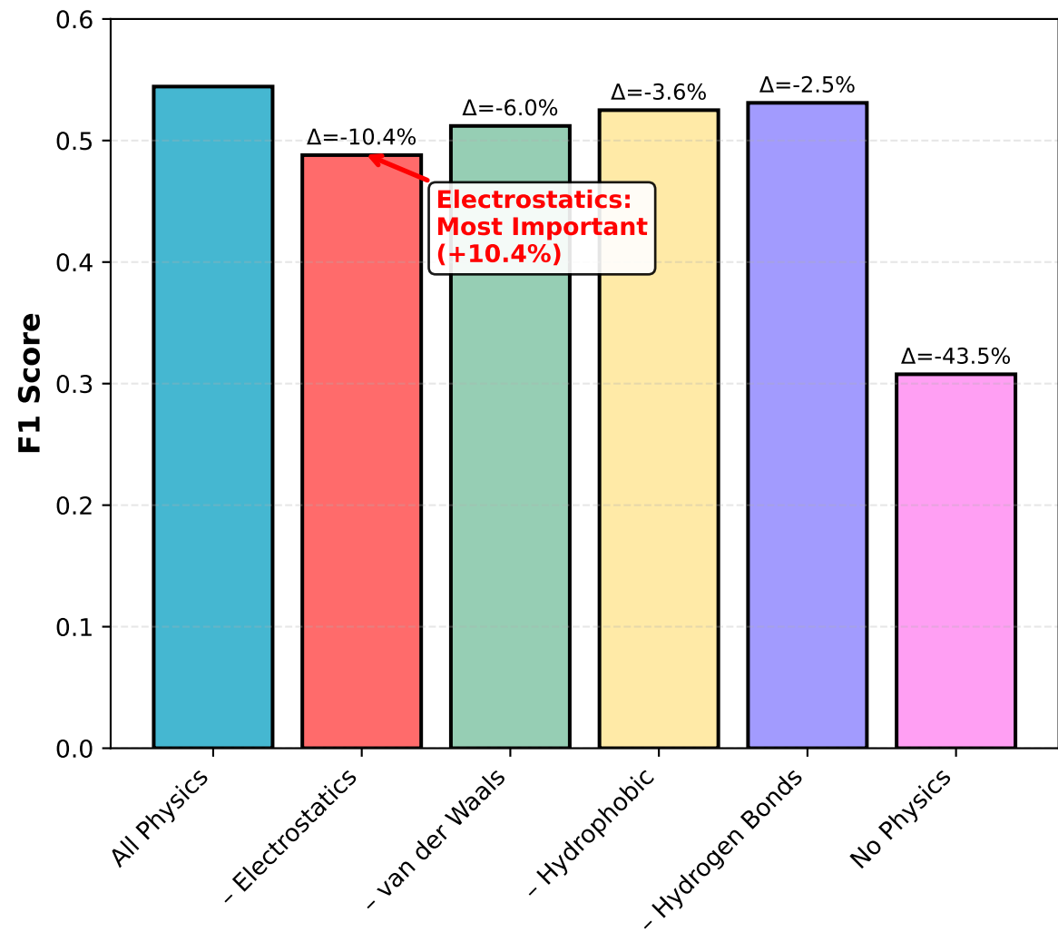
Physics Component Ablation Study
