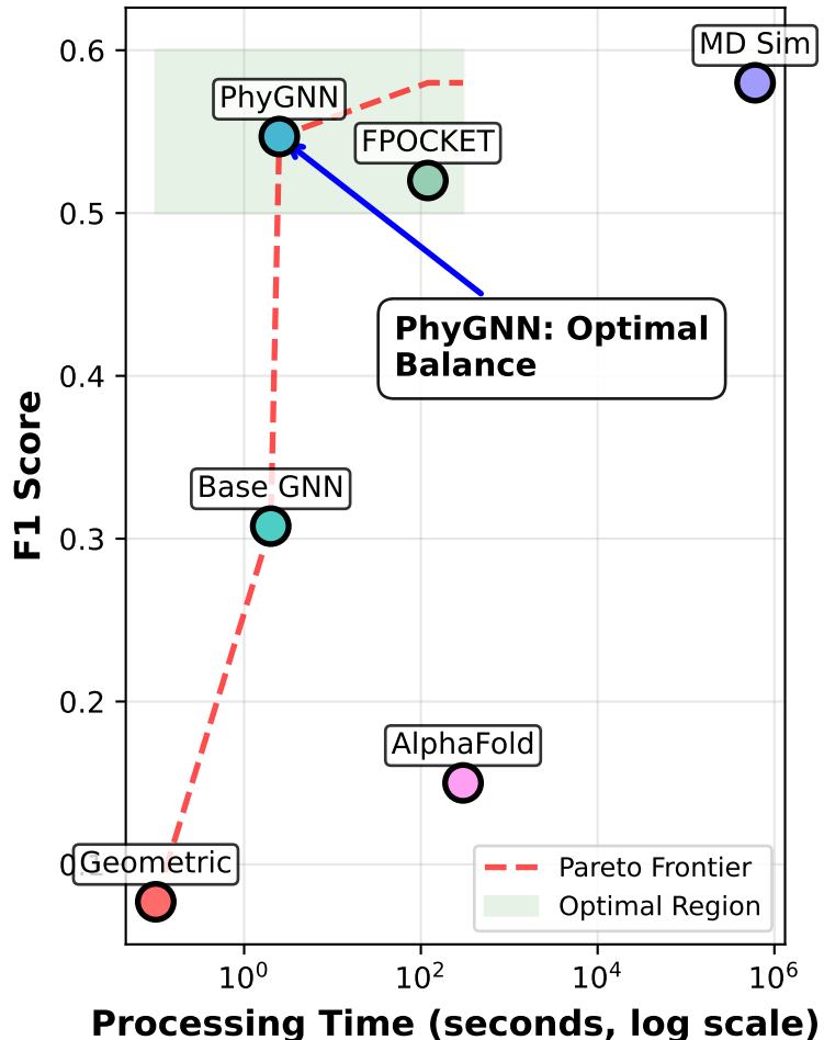
Speed-Accuracy Pareto Frontier
