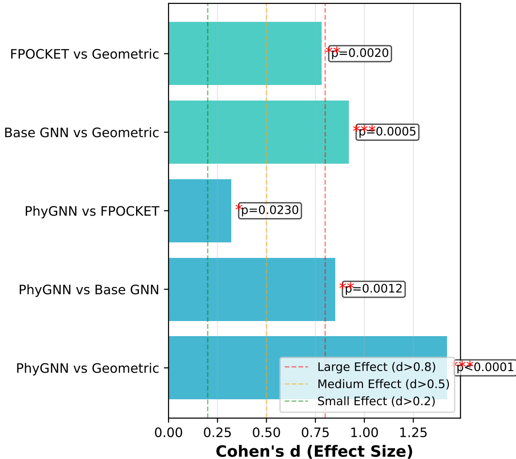
Statistical Significance Tests
