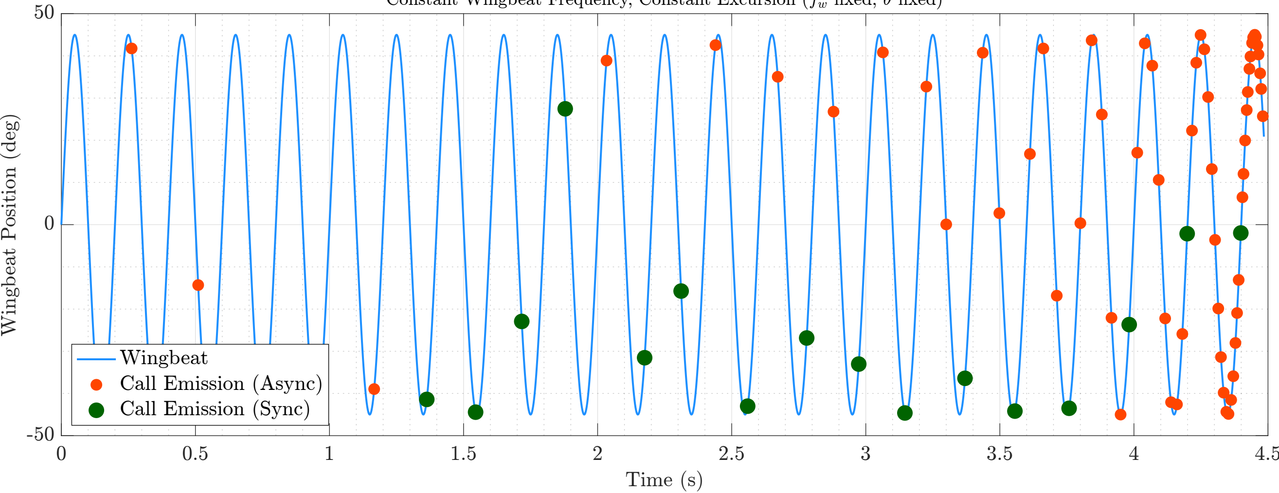
Constant Wingbeat Frequency, Constant Excursion ( f_w fixed, \theta fixed)
