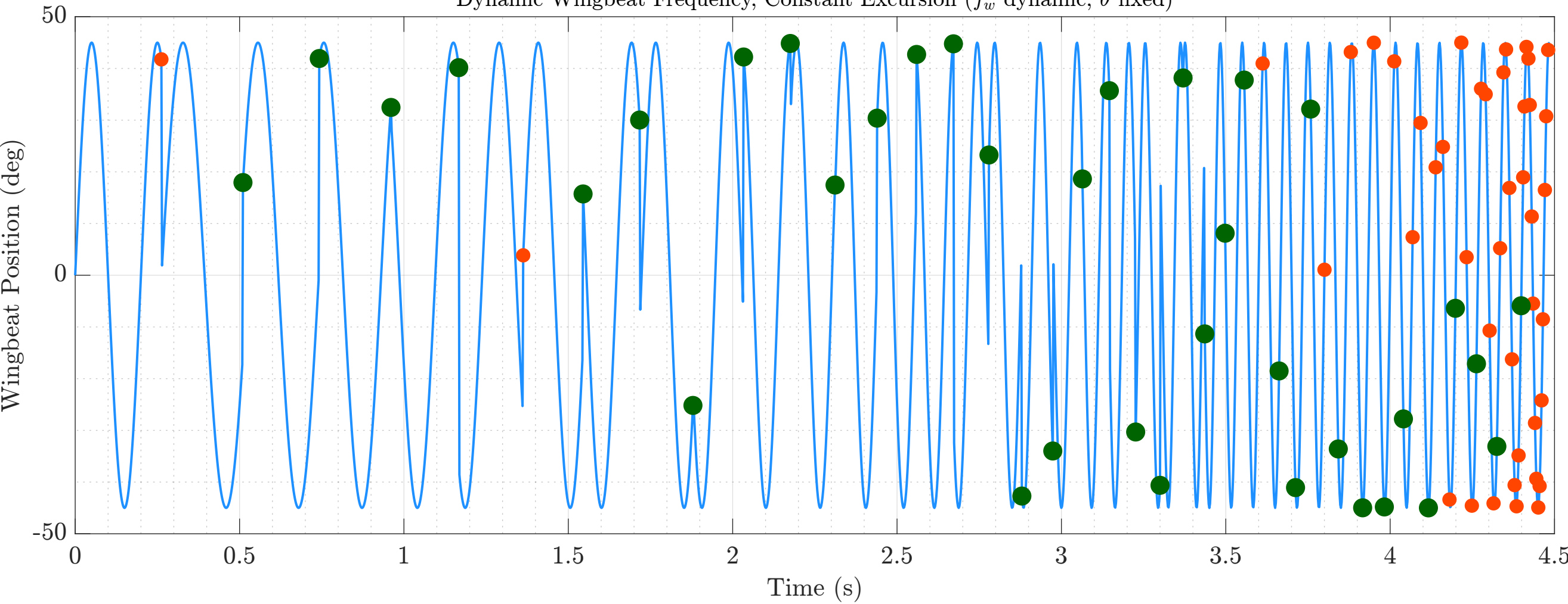
Dynamic Wingbeat Frequency, Constant Excursion ( f_w dynamic, \theta fixed)
