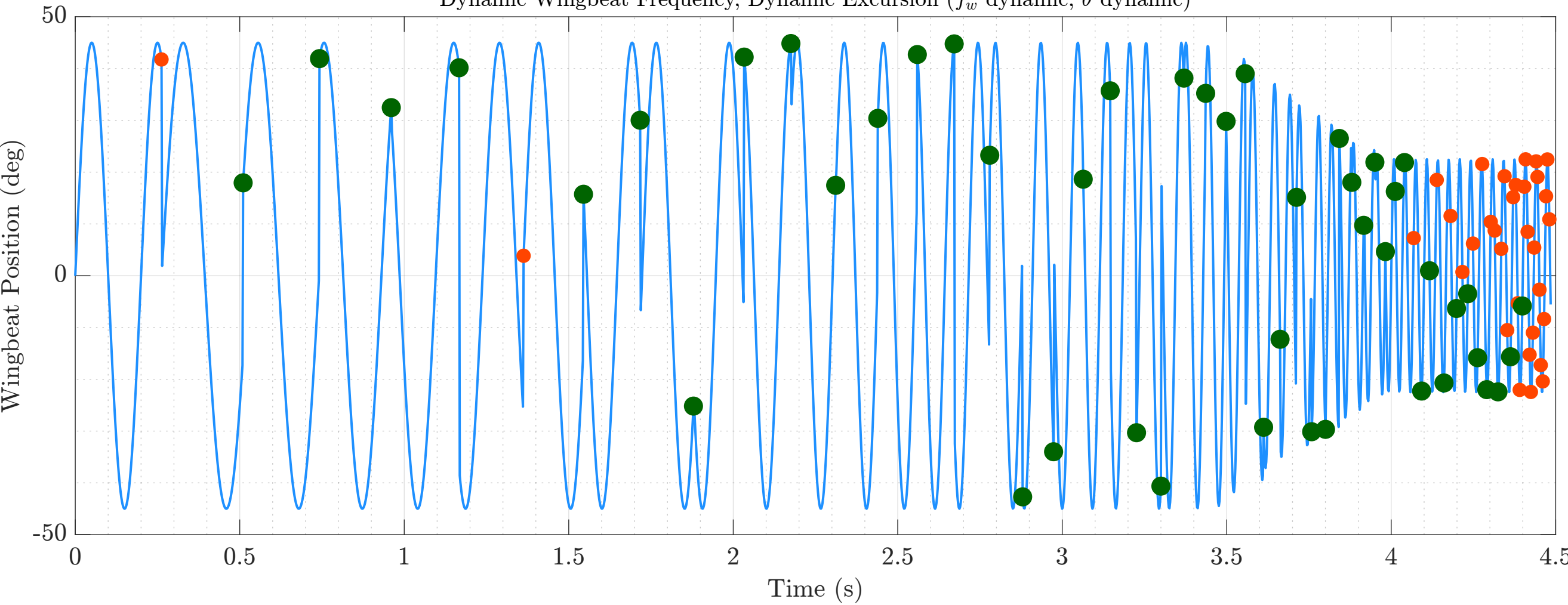
Dynamic Wingbeat Frequency, Dynamic Excursion ( f_w dynamic, \theta dynamic)
