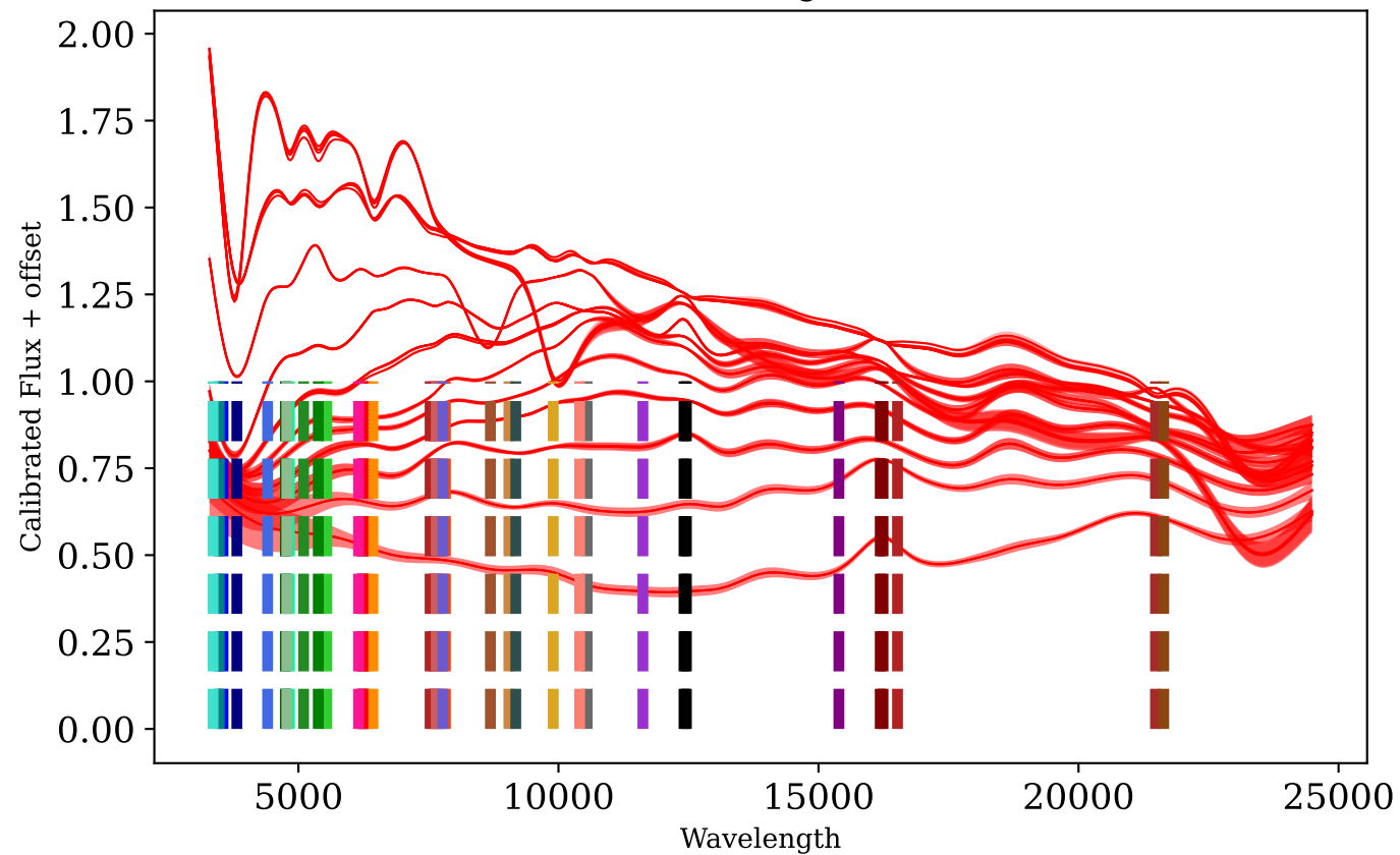
AT2017gfo
