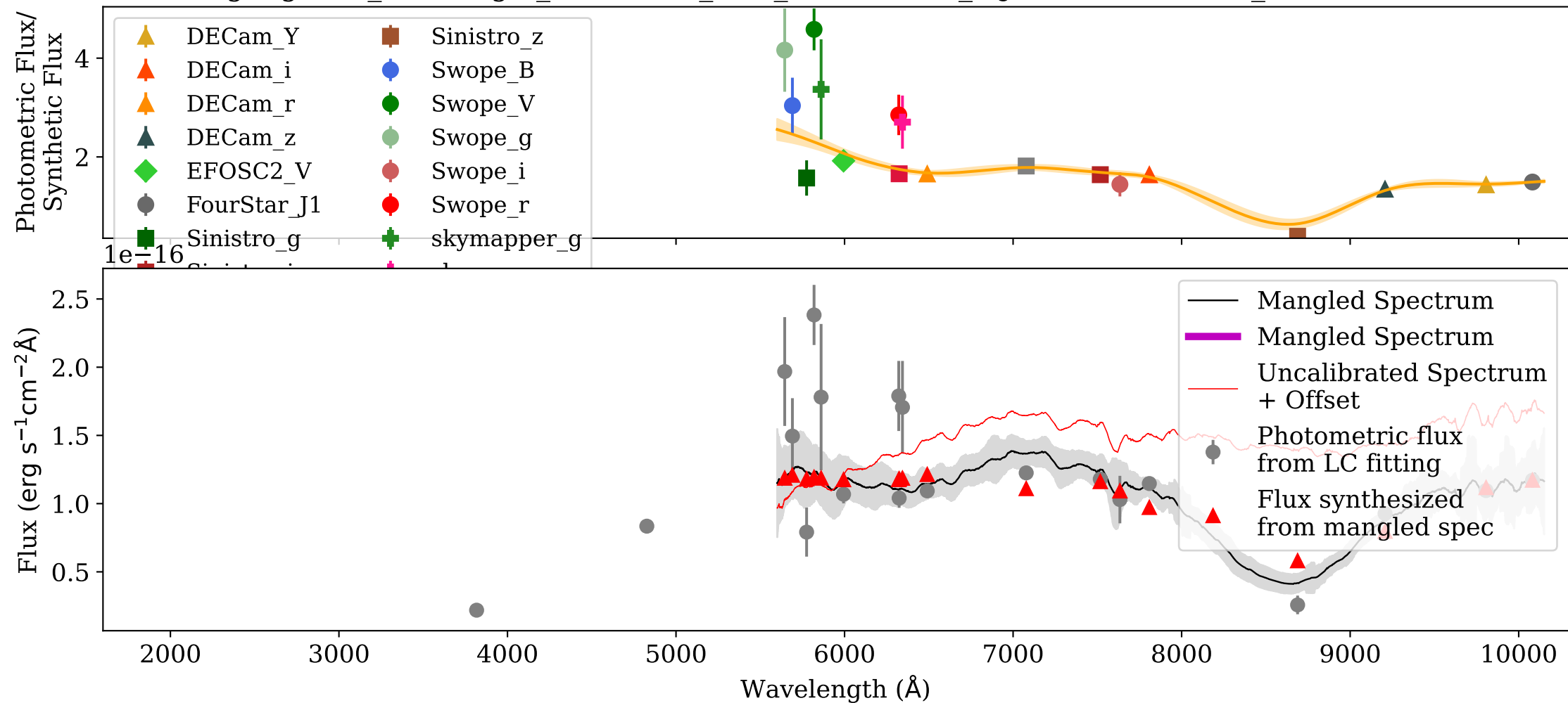
Mangling: VIS_AT2017gfo_ENGRAVE_v1.0_XSHOOTER_MJD-57984.969003_Phase+2.42d.dat
