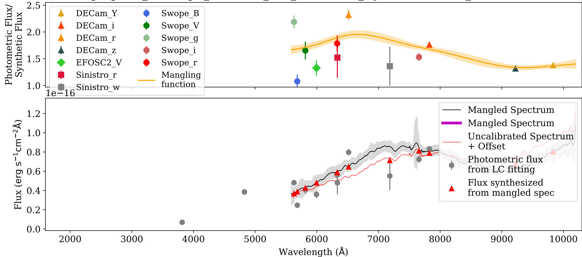
Mangling: VIS_AT2017gfo_ENGRAVE_v1.0_XSHOOTER_MJD-57985.974003_Phase+3.41d.dat
