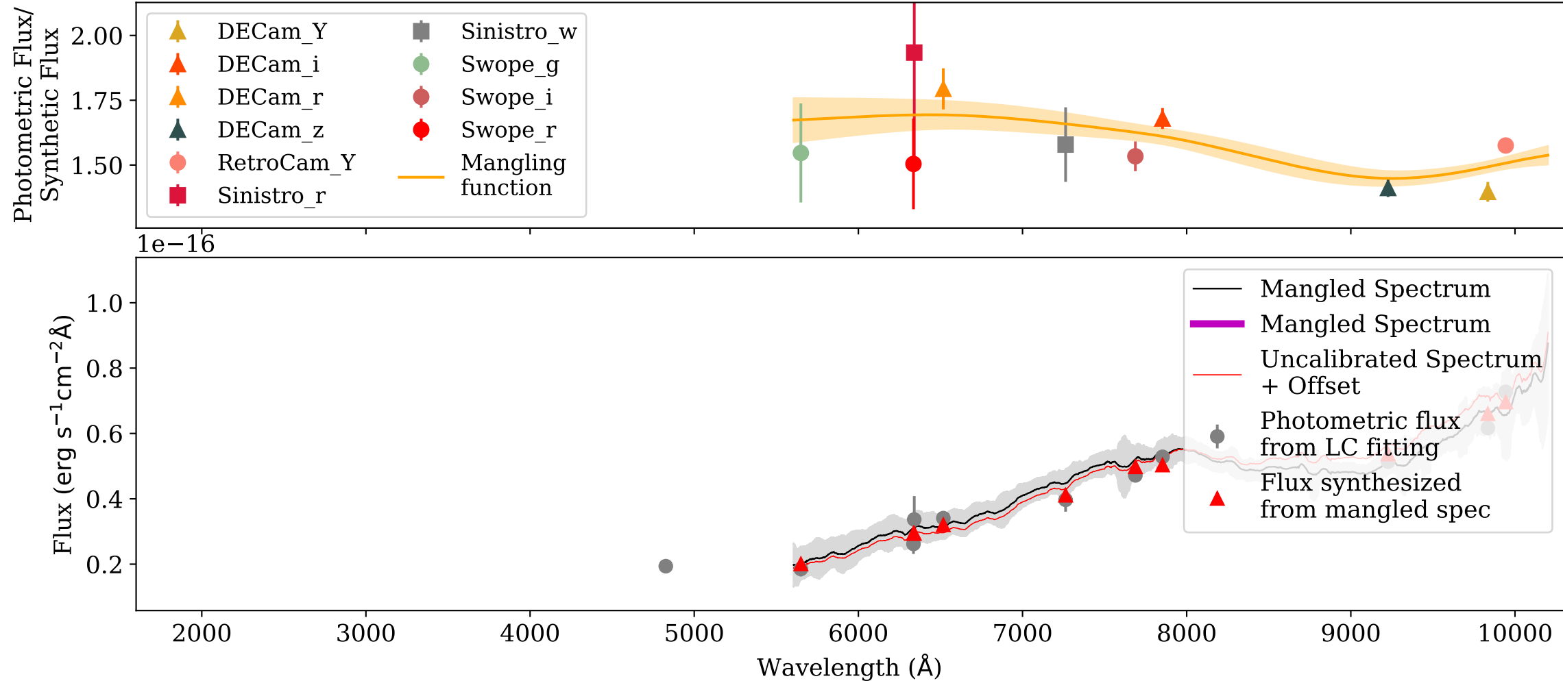
Mangling: VIS_AT2017gfo_ENGRAVE_v1.0_XSHOOTER_MJD-57986.974003_Phase+4.40d.dat
